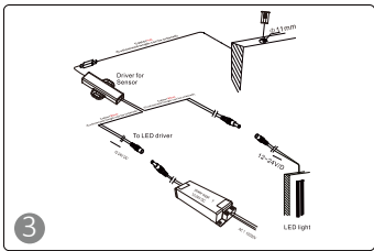
3 Connect the sensor and power supply as correct way.
