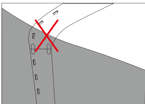
Distortion(Wrong)
