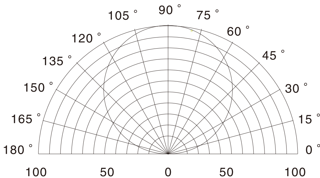
Radiation diagram
