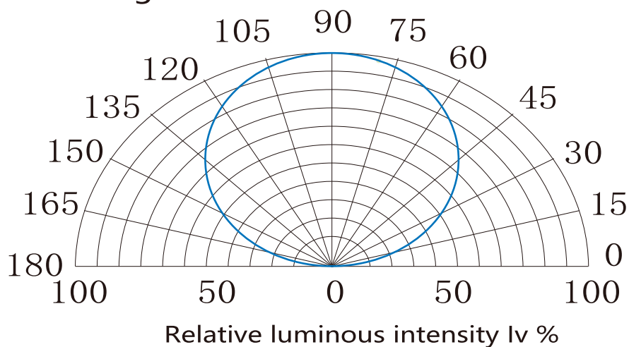
Radiation diagram
