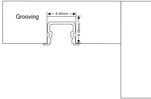
Recessed installation
