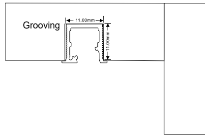
Recessed installation
